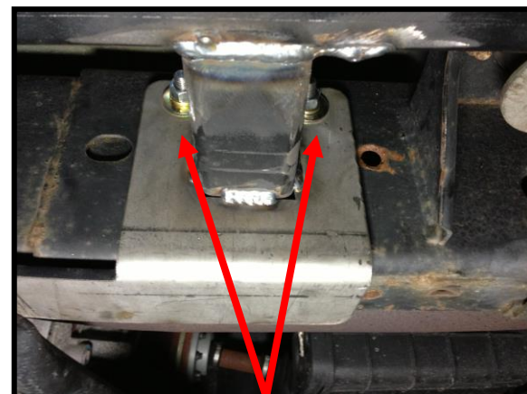
Figure 3 – U-Bolts Installed & Fastened
